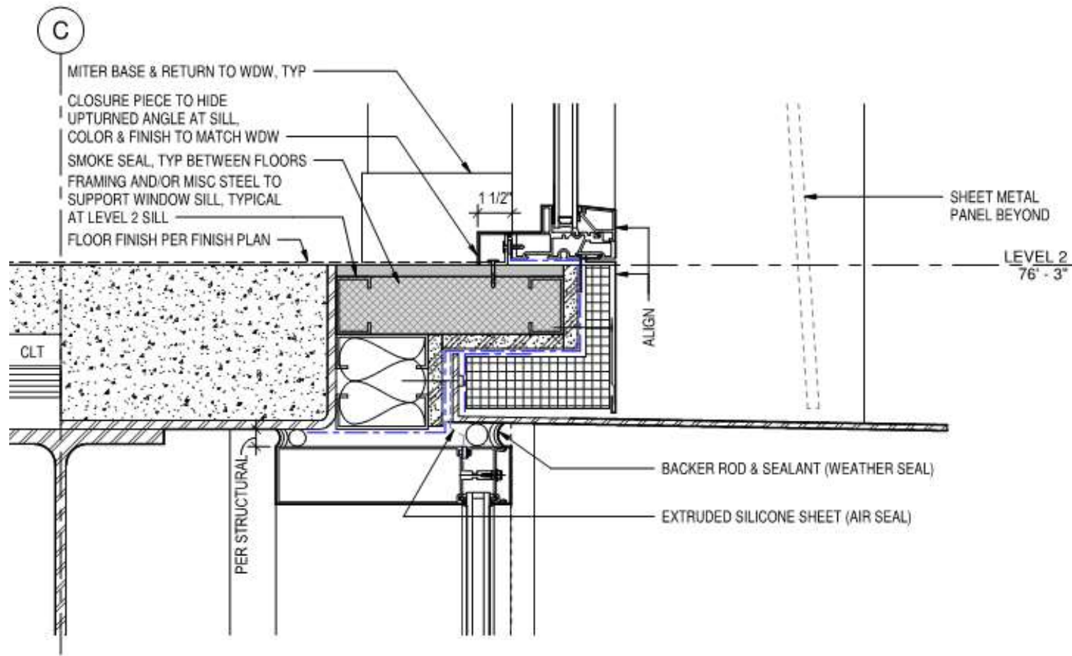
24 SECTION - WINDOW SILL AT CURTAINWALL 3" = 1'-0"
