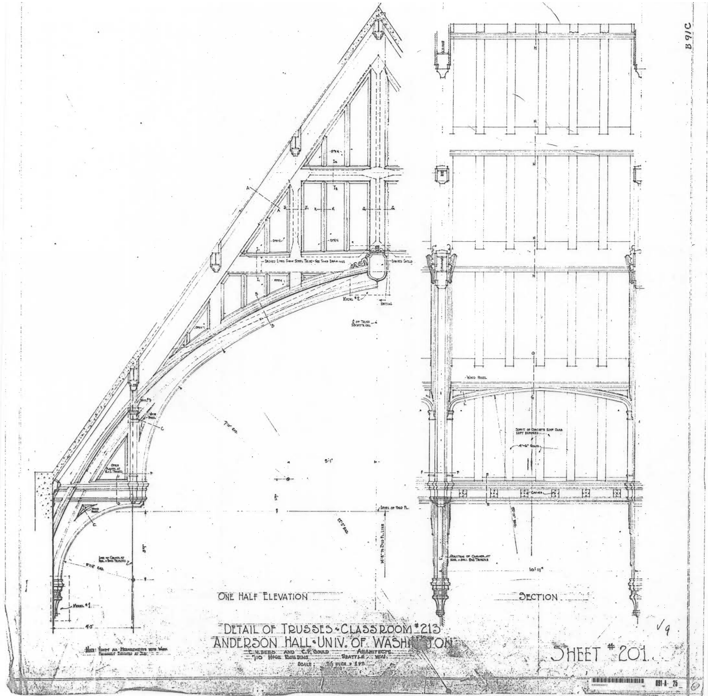
Figure 95. Lecture Hall, truss details.
